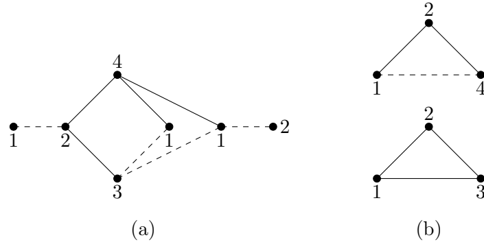
Figure 5.3: Signified coloring.
