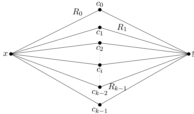
Figure A.2: A planar embedding of und(H)
