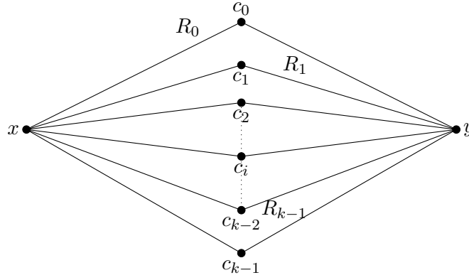
Figure 3.8: A planar embedding of und(\vec{H})
