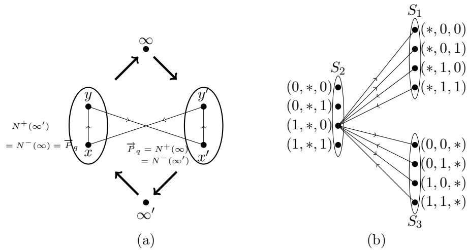
Figure 3.2: (a) The Tromp graph \vec{T}_{2q+2} (thick arrow means all the arcs are to/from \infty or \infty' from/to the vertices inside the ellipse. (b) Adjacency of a vertex of the Zielonka graph \vec{Z}_3 .)
